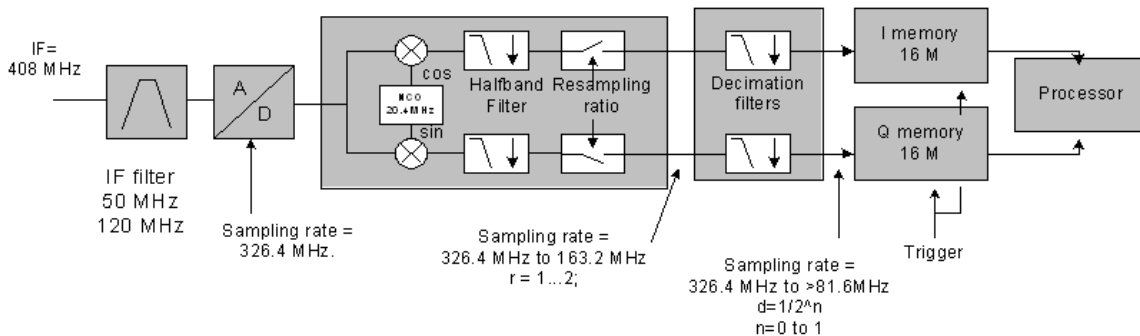
Block diagram of the R&S FSQ's signal processing at sampling rates >81.6 MHz
