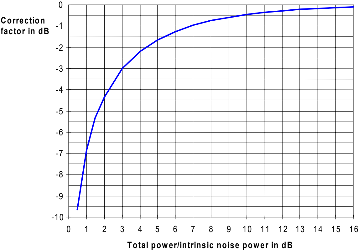
Fig. 2-13 Correction factor for measured noise power as a function of the ratio of total power to the intrinsic noise power of the Signal Analyzer.
