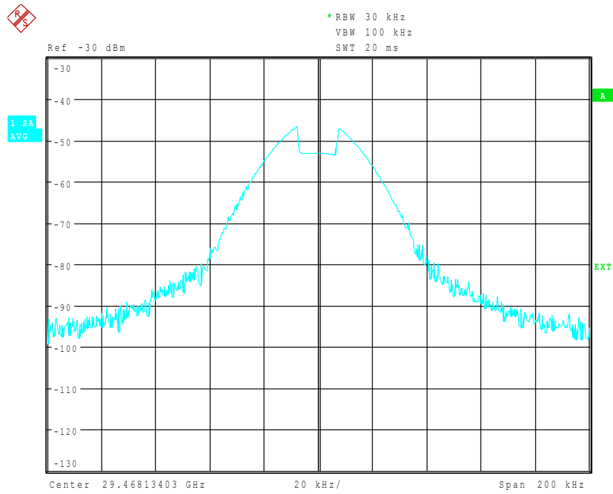
Fig. 4-39 Signal as in Fig. 4-37, but with the use of AUTO ID
