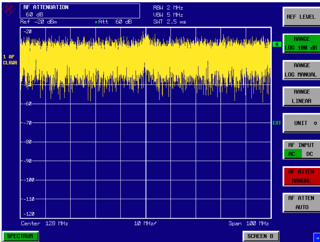
Fig. 2-9 Sinewave signal with low S/N ratio. The signal is measured with the autopeak detector and is completely swamped by the intrinsic noise of the Signal Analyzer.
