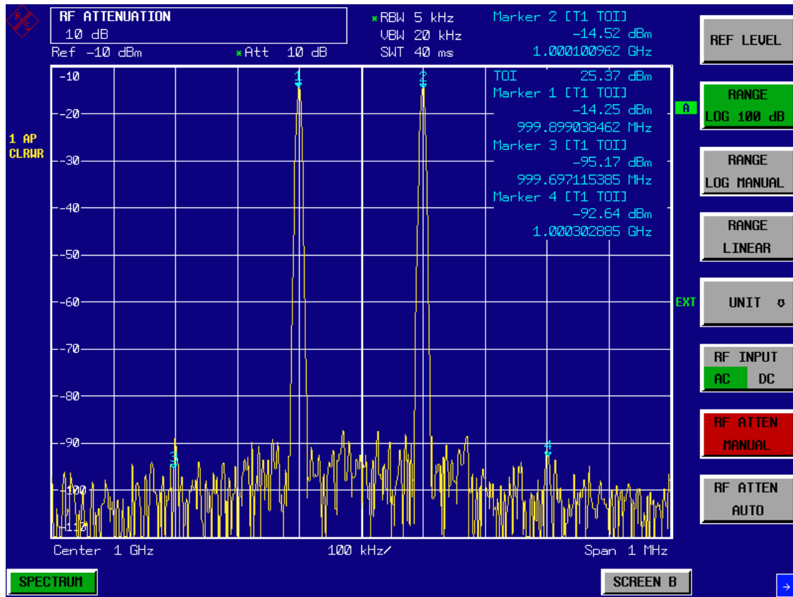
Fig. 2-4 If the RF attenuation is increased, the R&S FSQ's intrinsic intermodulation products disappear below the noise floor.
