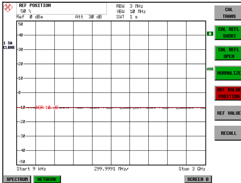
Fig. 4-22 Measurement with REF VALUE -10 dB and REF VALUE POSITION 50%
