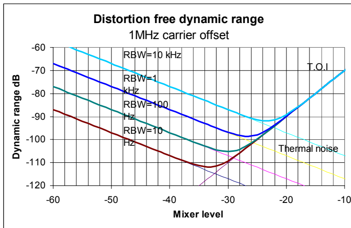
Fig. 2-5 Intermodulation-free range of the R&S FSQ as a function of level at the input mixer and the set resolution bandwidth (useful signal offset = 1 MHz, DANL = -157 dBm /Hz, TOI = 25 dBm; typical values at 2 GHz)
