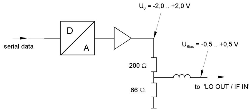
Fig. 4-35 Bias circuit of the Signal Analyzer
