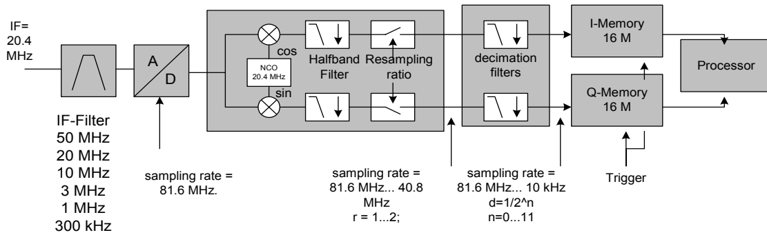
Fig. 6-1 Block diagram illustrating the R&S FSQ signal processing
