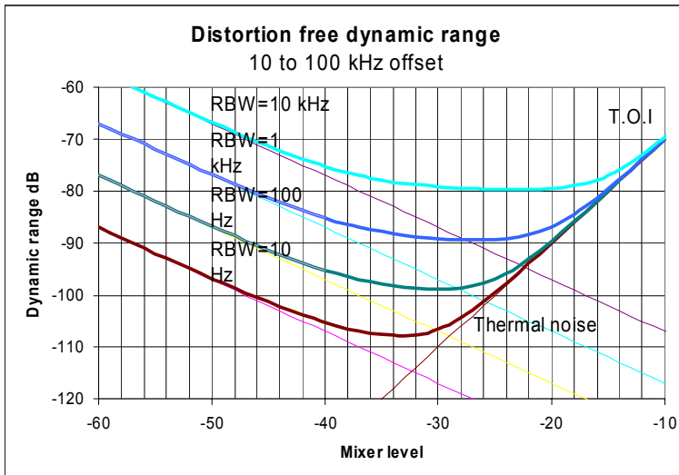
Fig. 2-6 Intermodulation-free dynamic range of the R&S FSQ as a function of level at the input mixer and of the selected resolution bandwidth (useful signal offset = 10 to 100 kHz, DANL = -157 dBm /Hz, TOI = 25 dBm; typical values at 2 GHz).
