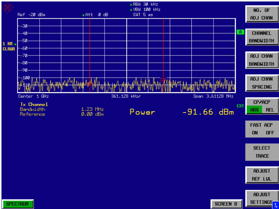
Fig. 2-14 Measurement of the R&S FSQ's intrinsic noise power in a 1.23 MHz channel bandwidth.
