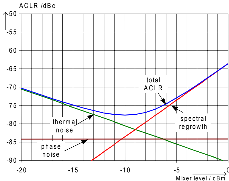
Fig. 2-34 The R&S FSQ's dynamic range for adjacent channel power measurements on W-CDMA uplink signals is a function of the mixer level.
