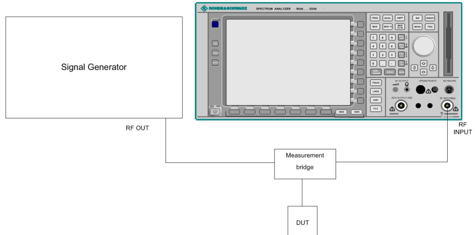
Fig. 4-27 Test setup for transmission measurement
