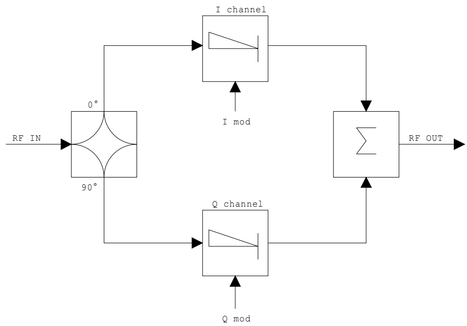
Fig. 4-26 I/Q modulation
