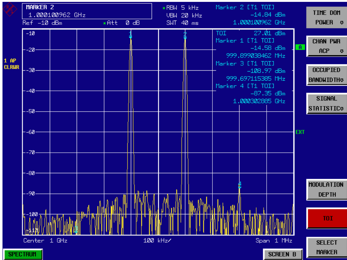
Fig. 2-3 Result of intrinsic intermodulation measurement on the R&S FSQ. The 3 rd order intercept (TOI) is displayed at the top right corner of the grid
