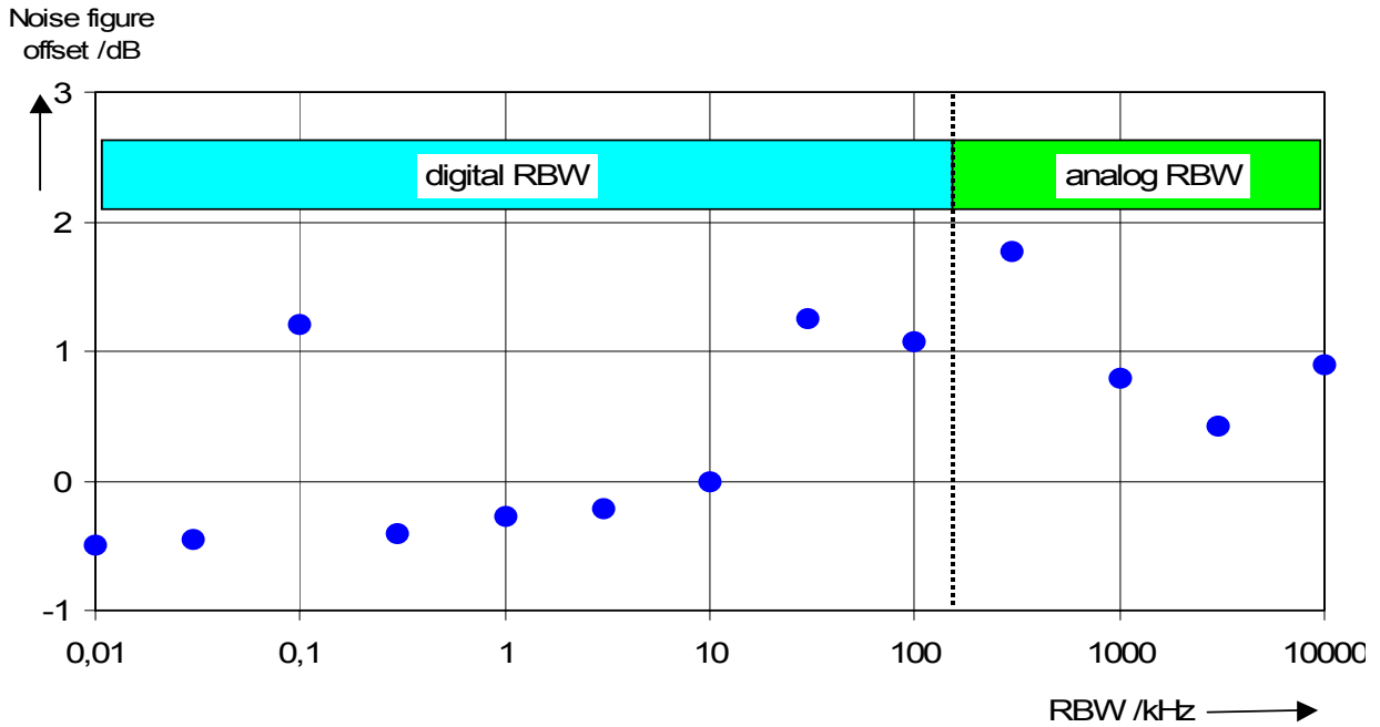
Fig. 2-8 Change in R&S FSQ noise figure at various bandwidths. The reference bandwidth is 10 kHz
