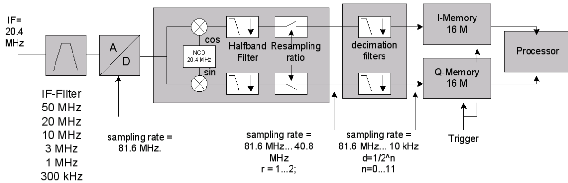
Fig. 7-3 Block diagram illustrating signal processing by the Signal Analyzer
